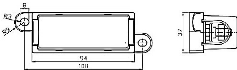
Fuse Holder for MEGA fuse
