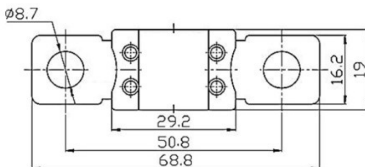
MEGA fuse
